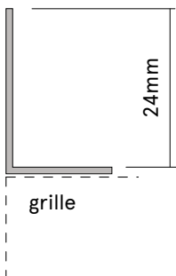
LV2516 STEEL FLANGE
