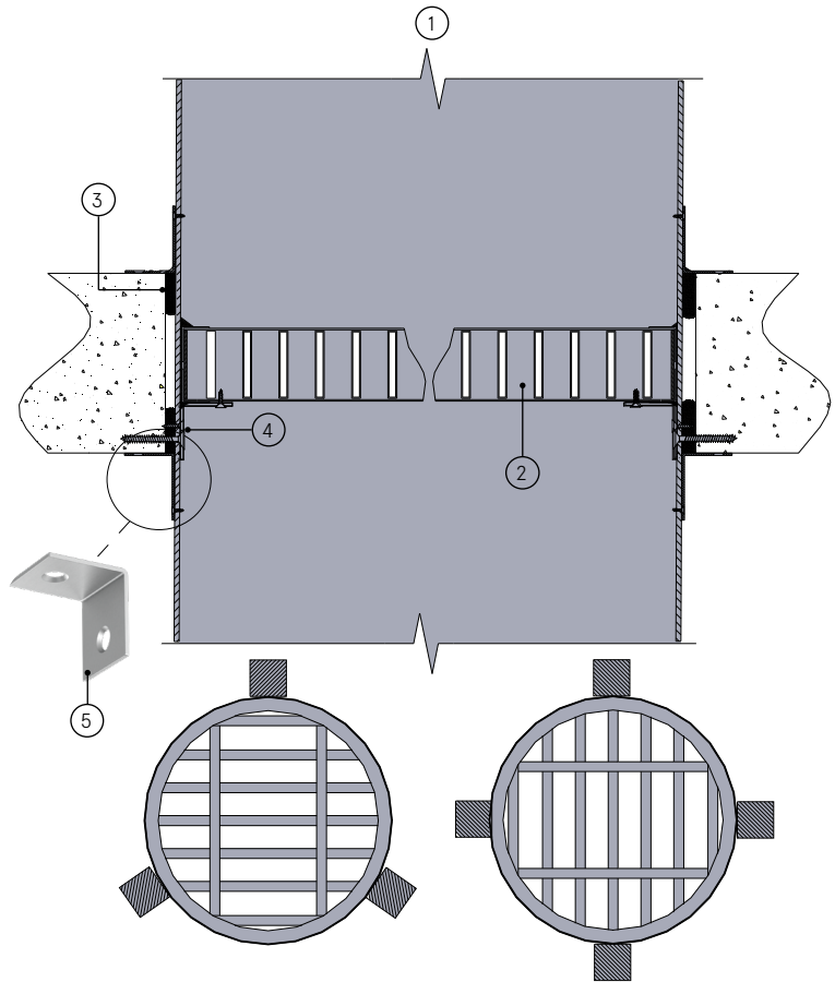
FIXING OPTION 1
