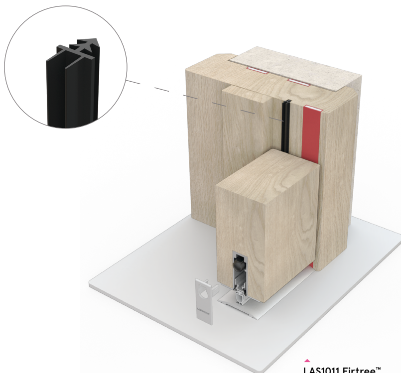
▲ LAS1011 Firtree™ Shown with fire seal as referenced in CNA/F14171 (shown with LAS8005 si + LAS4002)
