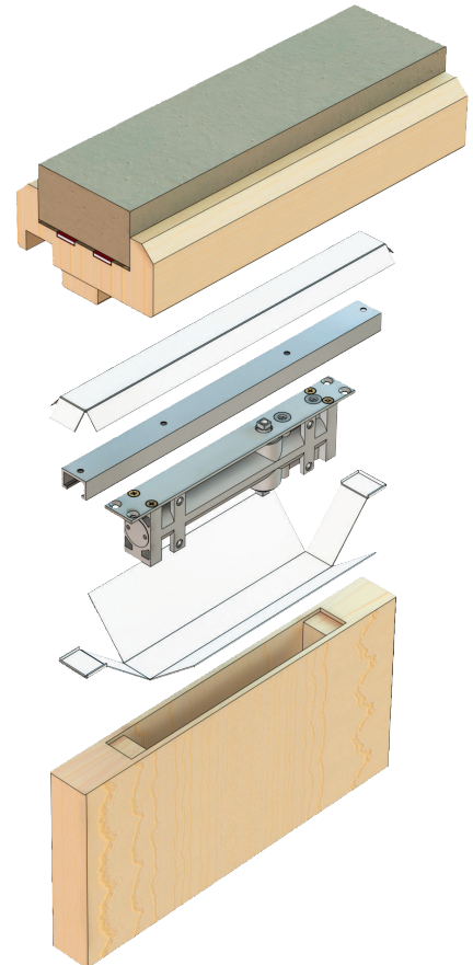
Concealed door closer protection kit ▶
