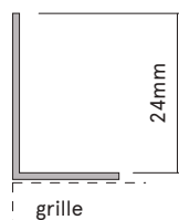
LV2516 steel flange
