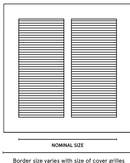
AIR TRANSFER GRILLE / COVER GRILLE SELECTOR (MM)
