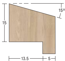
Glazing bead For 44mm thick doors or rebated screen frames.
