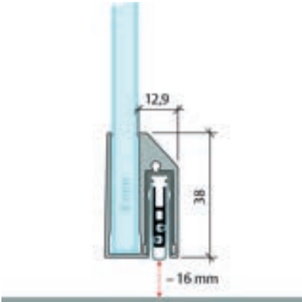
Planet KG-A8
