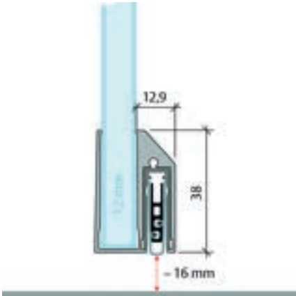
Planet KG-A12
