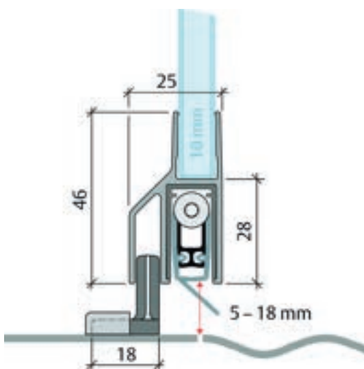
Planet KG-SL10
