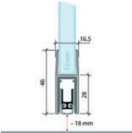
Planet KG-F12
