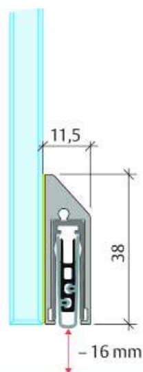
Planet KG-S Narrow Drop Seal
