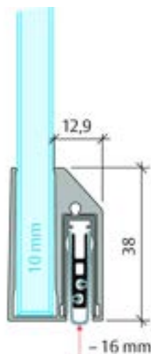
Planet KG-A10 Narrow Drop Seal
