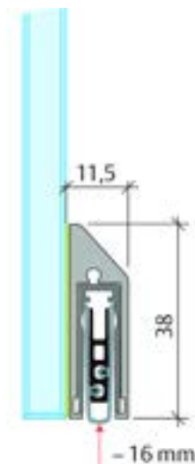
Planet KG-SM Set Narrow Drop Seal
