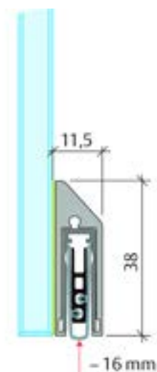
Planet KG-S Narrow Drop Seal
