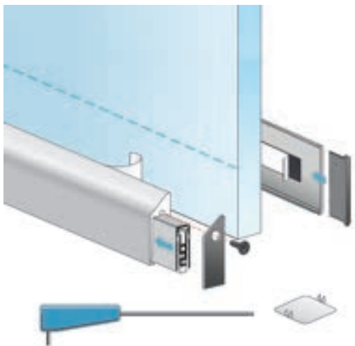
Planet KG-SC Narrow Drop Seal
