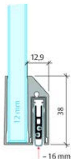
Planet KG-A12 Narrow Drop Seal
