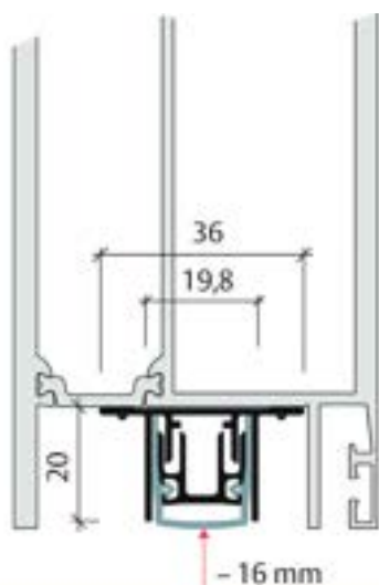
Planet RO Drop Seal
