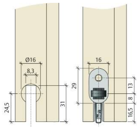
Planet Pivot Drop Seal
