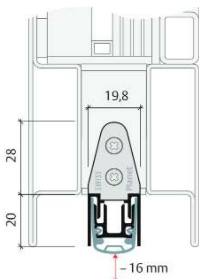
Planet MF-PLUS Drop Seal
