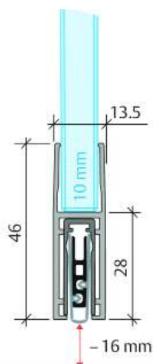
Planet KG-F10 Drop Seal
