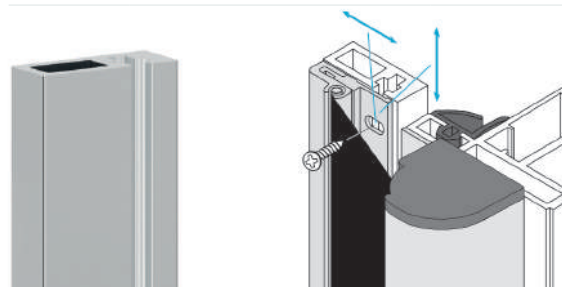
Base profile FSR RG1, for glass doors
