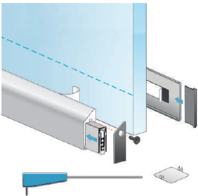
Planet KG-SC narrow
