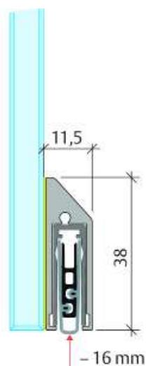
Planet KG-S Narrow Drop Seal
