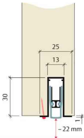
Planet FT Drop Seal
