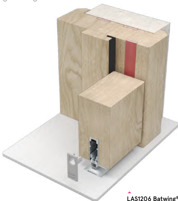
LAS1206 Batwing® Shown with fire seal as referenced in CNA/F14171 (also shown with LAS8001 si)
