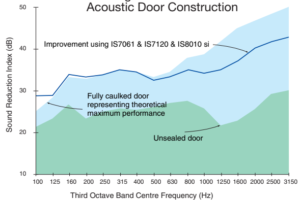
High Performance Acoustic Door Construction
